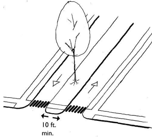
One-way driveways with minimum 10 ft median.
